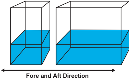
Diagram 28: Tank breadth and the free surface effect
