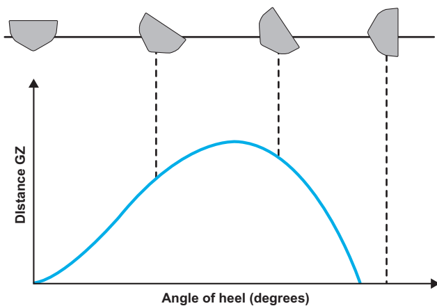
Diagram 19: The GZ curve
