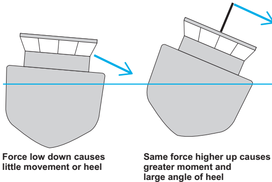
Diagram 10: The effect of height on the angle of heel
